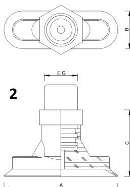
Vacuum Cup oval (complete) Vakuumsauger oval (komplett) Ventosa ovale (completa) Ventouse ovale (complet) Ventosa oval (completa)
