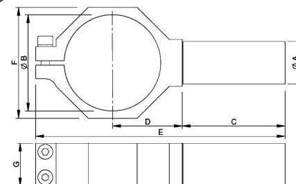
Mounting Bracket MR - Klemstück MR
